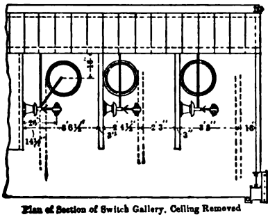
FIG. 13.— 60,000-VOLT DISCONNECTING SWITCH.
